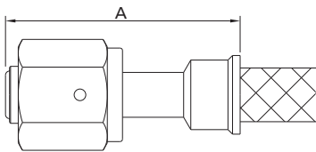
Female FR Metal Gasket Face Seal Fittings Swivel
