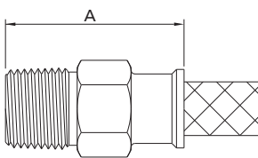
Male Pipe Threads, NPT
