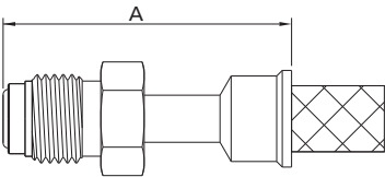
Male FR Metal Gasket Face Seal Fittings Swivel
