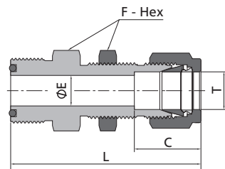
FO Body to Bulkhead Tube Fitting
