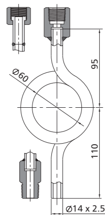
WS Series
