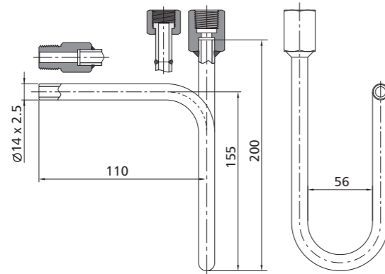
UWS Series
